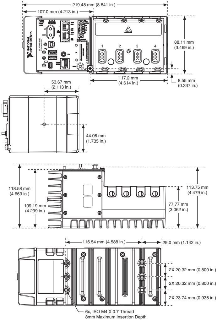
Figure 1. NI cDAQ-9132 Dimensions
