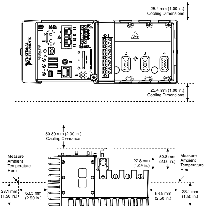
Figure 2. NI cDAQ-9132 Temperature, Cooling, and Cabling Dimensions
